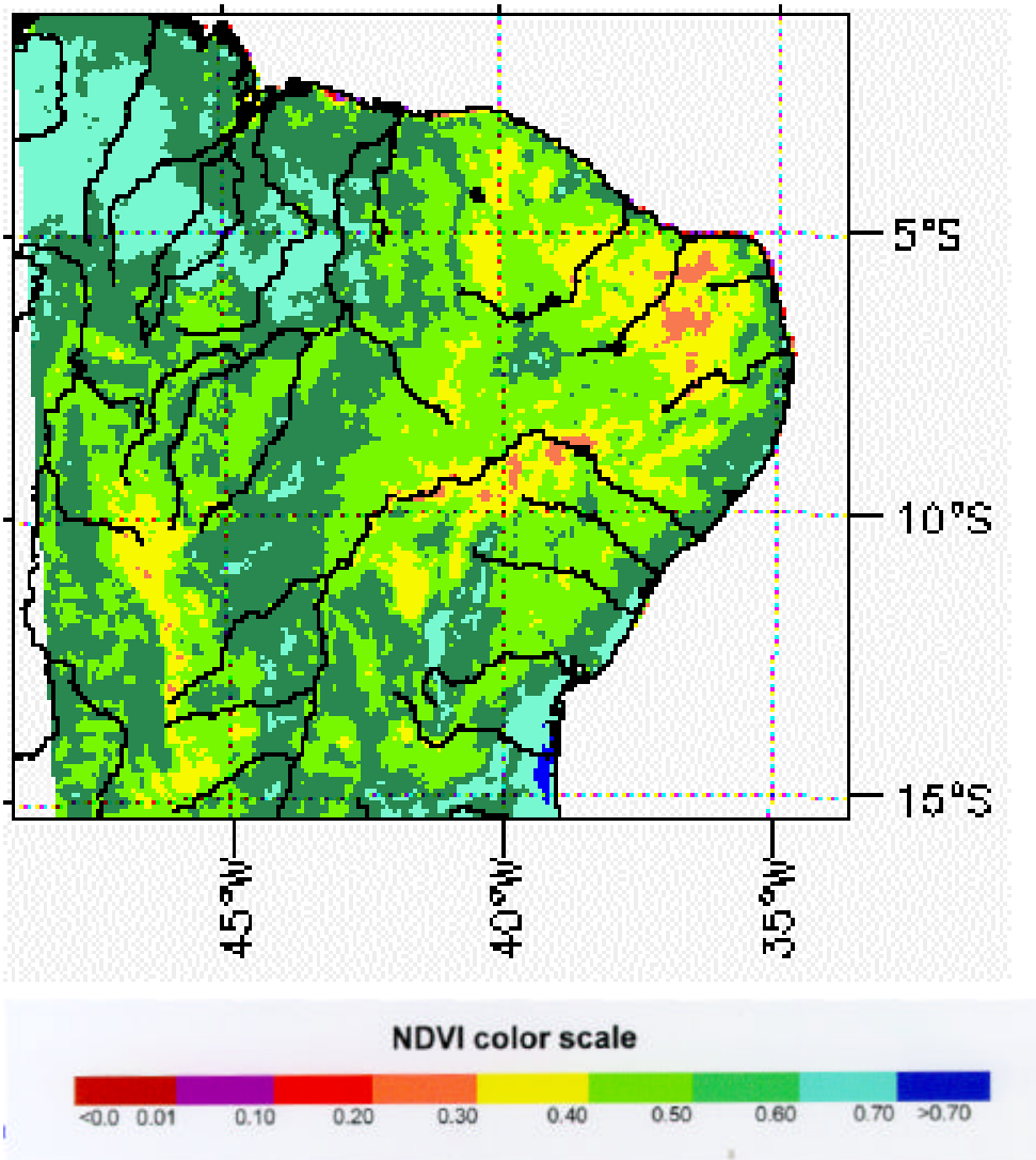
Figure 1 - NDVI monthly average map of Northeast Brazil (NDVI data: 07/81 to 06/93).
